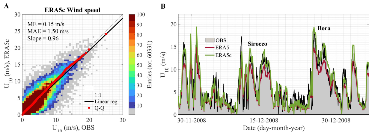
Figure 10. Performance of ERA5c wind speed ( U_{10} , in m/s). Comparison with in situ observations (OBS) in the northern Adriatic Sea (Acqua Alta oceanographic platform, AA) during years 2004–2010. (A) Scatter diagram (color shade, linear scale) and quantile-quantile plot (Q-Q, red markers) at 1%-interval up to 99th and 0.1% interval above. Mean error (ME), mean absolute error (MAE), and slope (Slope) of the line of best fit (thick black) are shown in the plot area. The dashed black line indicates the perfect 1:1 match between datasets. (B) Example of time series comparison between measured (gray area), ERA5 (red line), and ERA5c (green line) speeds. Two Sirocco and Bora storms are indicated in the plot area.
