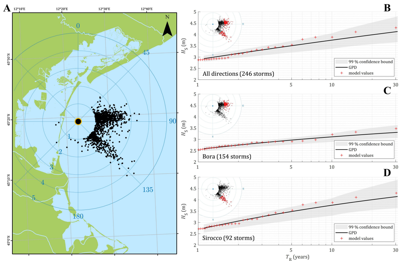
Figure 14. The long-term wave climate offshore the Venice lagoon (the northern Adriatic Sea; see Figure 1) for the present-day period 1981–2010. (A) Geographical position of the location of interest (black dot at the center of the polar grid) and distribution (small black dots) of H_s (radius, discretized every 1 m) and peak direction of propagation (angle, clockwise from the north). The long-term distribution of the POT ranked H_s values and associated empirical return periods T_R (red crosses) for the overall sea states (B), Bora sea states (C), and Sirocco sea states (D). In the inset, the polar grid replicates with black dots the grid on panel (A), while the red dots identify the storms used for the extreme analysis of each dataset. The black line shows the generalized Pareto distribution (GPD) values and their confidence interval (shaded gray area).
