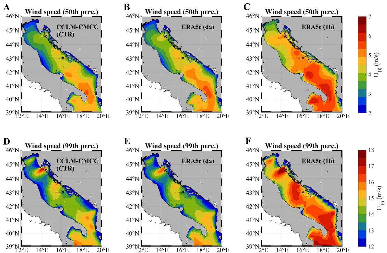
Figure 9. Wind speed climate over the Adriatic Sea and the northern Ionian Sea for the years 1981–2010. Average of annual 50th (A–C) and 99th (D–F) percentiles of U_{10} (in m/s). (A,D) CCLM-CMCC data from the control run (CTR); (B,E) daily averaged (da) ERA5c data; (C,F) ERA5c hourly data (1 h). For clarity, color scales change between (A–C) and (D–F).
